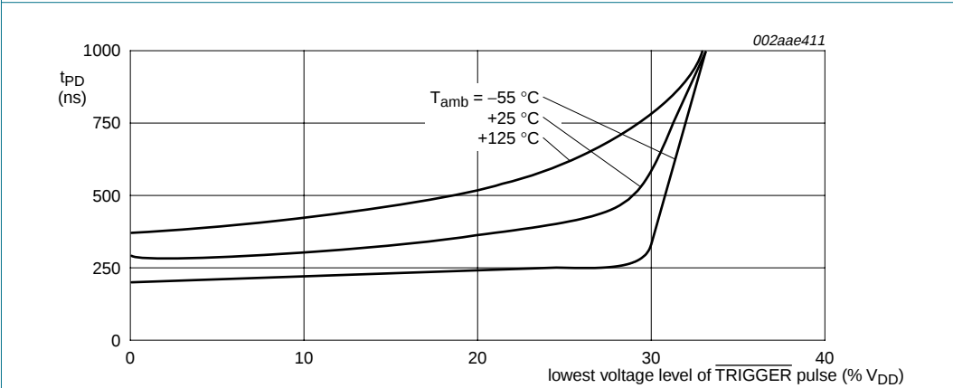
Fig 9. Propagation delay versus voltage level of \overline{\text{TRIGGER}} pulse ( V_{DD} = 5\text{ V} )
